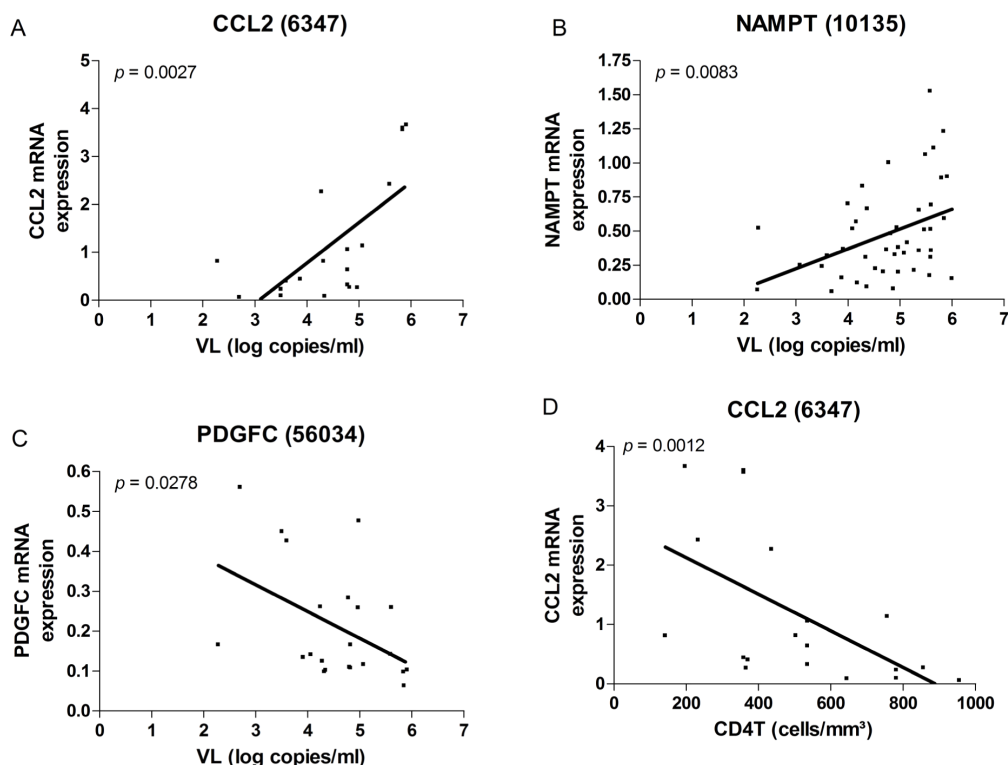
Figure 2 A-C) Correlation of mRNA gene expression in monocytes of therapy-naïve HIV patients, as assessed by RT-qPCR, with the viral load; D) Correlation of mRNA gene expression in monocytes of therapy-naïve HIV patients, as assessed by RT-qPCR, with the CD4 + T lymphocyte count - p -values for Spearman correlation testing are shown.
