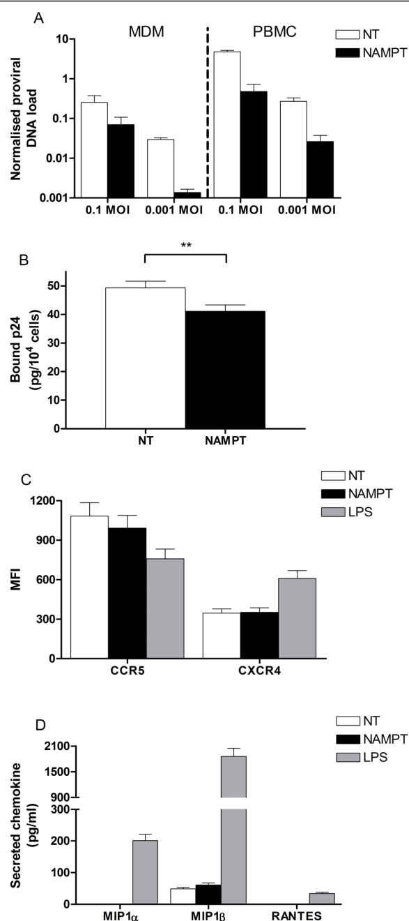
Figure 5 A) Levels of integrated proviral DNA in MDM and resting PBMC (pre-)treated with NAMPT (200 ng/ml) and infected with HIV Bal at 0.1 and 0.001 MOI, normalised to ERV-3, as assessed by RT-qPCR; B) viral binding to MDM, as quantified by p24 concentrations in cell lysates after 2 hours incubation and washing of the unbound virus; C) expression of CCR5 and CXCR4 on MDM treated 2 days with NAMPT (200 ng/ml) and LPS (100 ng/ml), as assessed by flow cytometry[39]; D) secretion of the \beta -chemokines MIP1 \alpha , MIP1 \beta and RANTES by MDM treated 2 days with NAMPT (200 ng/ml) and LPS (100 ng/ml), as assessed by CBA. MFI: mean fluorescence intensity.
