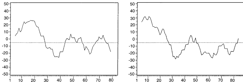
FIG. 3. Vpu protein of SIV CPZ-ANT . (A) Alignment of Vpu proteins from SIV CPZ-ANT , SIV CPZ-GAB , HIV-1 M, and HIV-1 O isolates using CLUSTAL W. Residues identical across all four sequences are indicated by *. The HIV-1 conserved Vpu motif is underlined. (B) Hydrophathy profiles of the SIV CPZ-ANT (left) and SIV CPZ-GAB (right) Vpu proteins were calculated according to Kyte and Doolittle (34). Positive scores are hydrophobic and the amino acid number is indicated on the X-axis.
