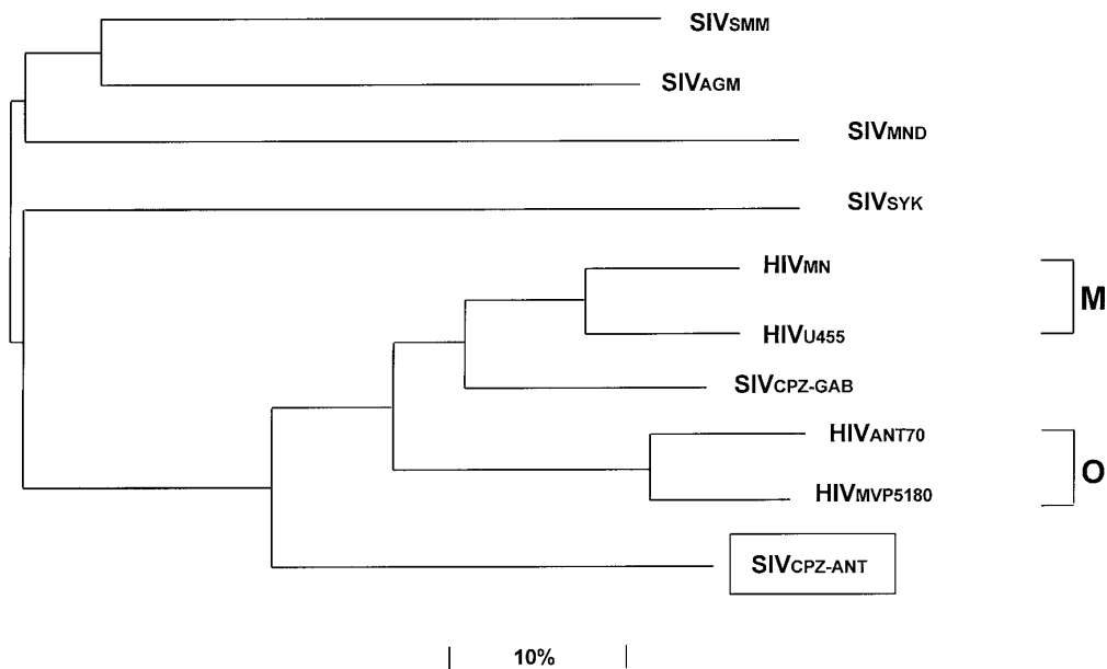
FIG. 1. Phylogenetic relationship of SIV CPZ-ANT to representative primate lentiviruses. Predicted Gag, Pol, and Env protein sequences were aligned and then concatenated; pairwise distances were calculated by Kimura's method (30), and the phylogeny was estimated by the neighbor-joining method (37) with 1000 bootstraps; these methods were implemented using CLUSTAL W (32). The tree is midpoint rooted. Horizontal branch lengths are to scale: the bar indicates 10% (0.10 amino acid replacements per site). All clusters within the HIV-1/SIV CPZ lineage were found in 100% of bootstraps. The same branching order within the HIV-1/SIV CPZ lineage was found in trees estimated from Gag, Pol, and Env proteins analyzed individually and in trees estimated by the maximum parsimony and weighted parsimony methods.
