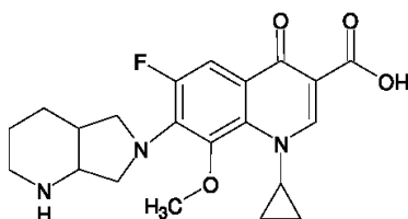
Moxifloxacin
